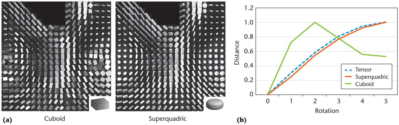
Figure 5. Evaluating tensor glyphs. (a) A superquadric and a cuboid glyph, used for visualizing the same tensor field. 6 The insets represent the diagonal tensor D . (b) Changes in the size of D and its superquadric and cuboid representations with respect to rotations around the tensor’s smallest eigenvector. The tensor size and the superquadric glyph’s appearance follow a similar trend; the cuboid glyph’s appearance differs. This suggests that superquadric glyphs better preserved the structure in the data.
